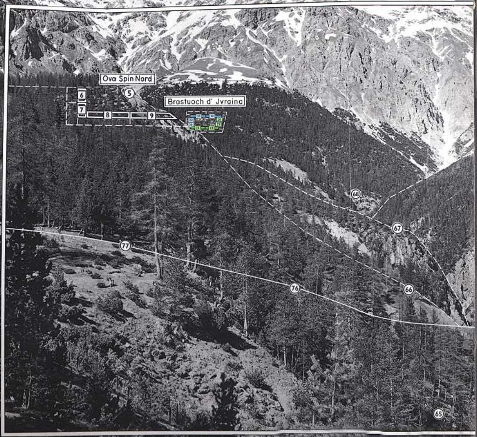
A7632 Mg I Ova Spin Strasse 30.1.70
